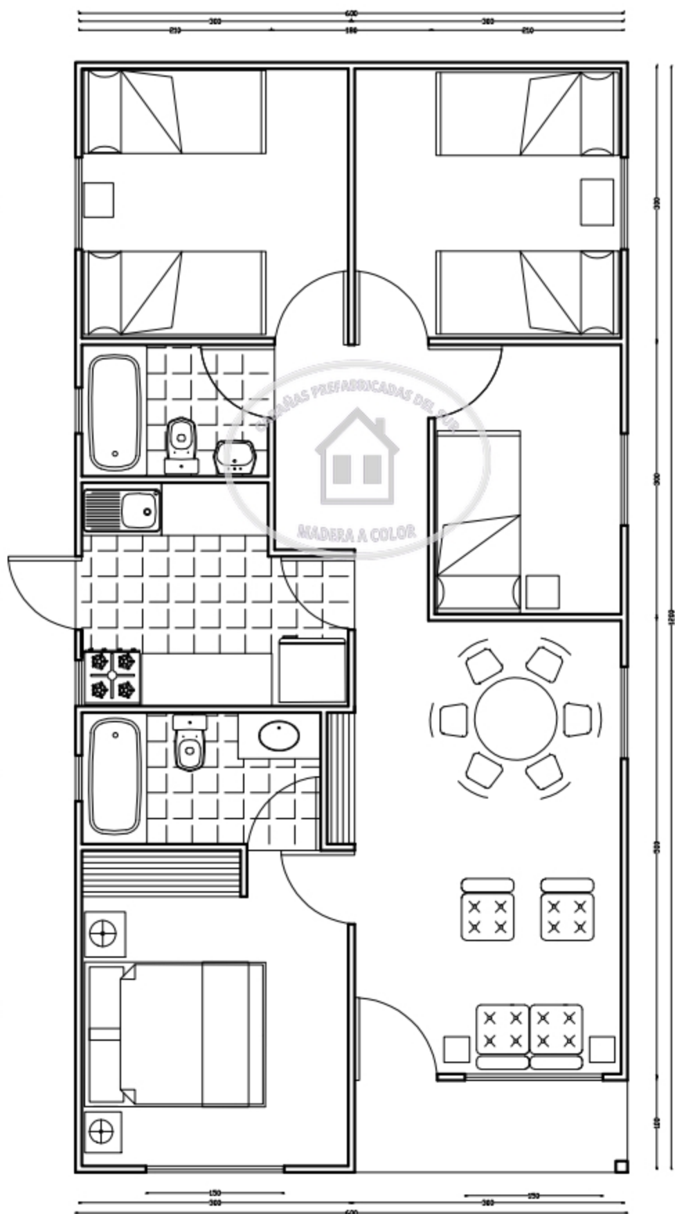
CABAÑA 72 m2 (6 X 12)
